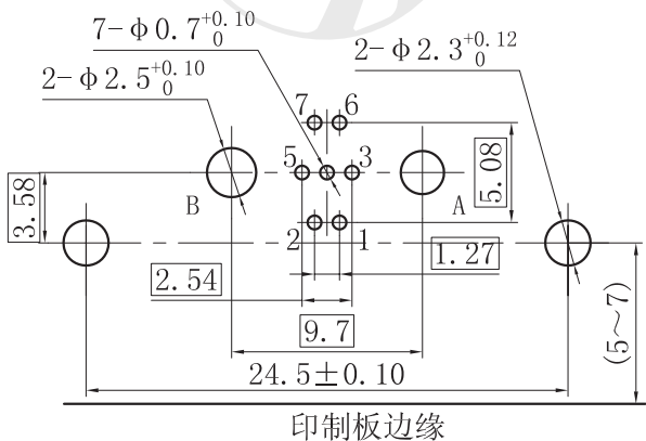
J30J09P02JSW01W10000弯插印制板开孔尺寸
