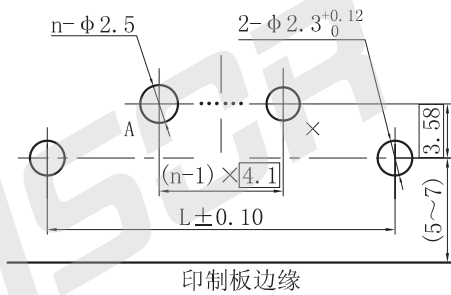
J30J□□P□□0P000W10000弯插印制板开孔尺寸
