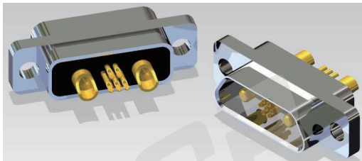
J30J 09P02 K P S00 S0 000 0
