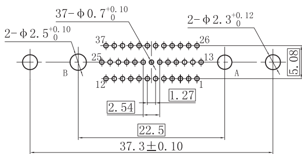
J30J39P02JSN01N10000直插印制板开孔尺寸
