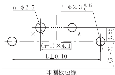
J30J□□P□□0S000W10000弯插印制板开孔尺寸
