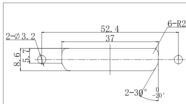
100 芯板后安装开孔尺寸
