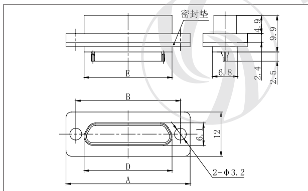
J30JM1-9~37ZKS
