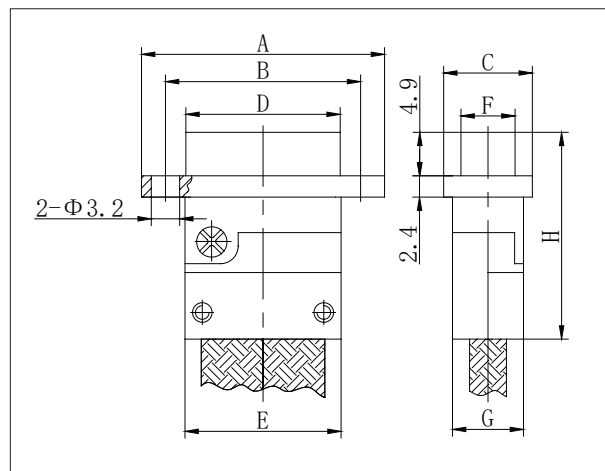
J30J-9~100ZK-GAQ
