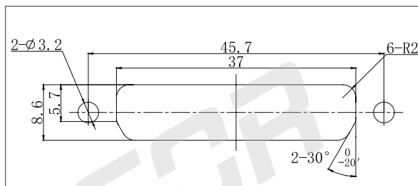
100 芯板后安装开孔尺寸
