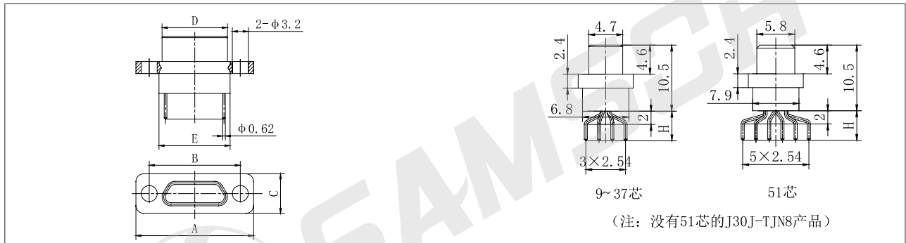
J30J-9~51TJN4/J30J-9~37TJN8
