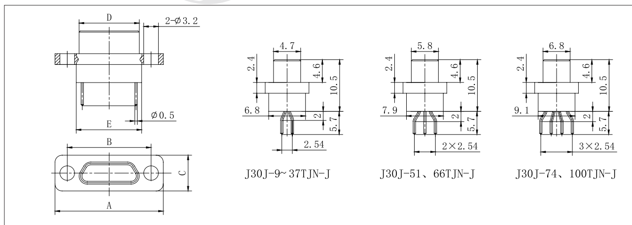
J30J-9~100TJN-J
