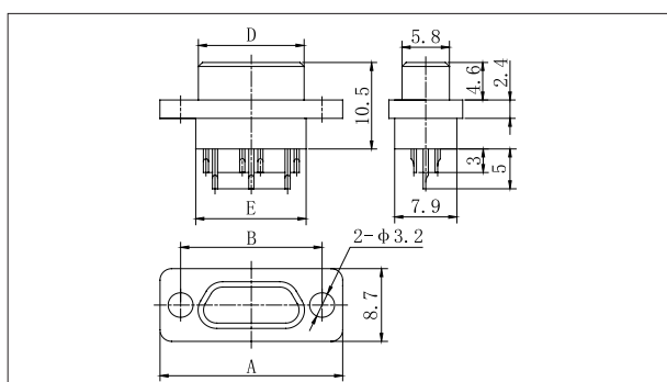
J30J-51, 66TJS
