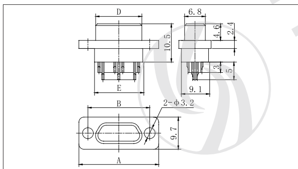
J30J-74, 100TJS
