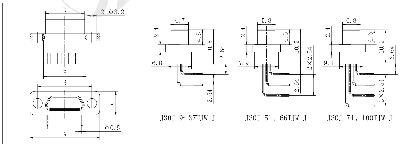
J30J-9~100TJW-J
