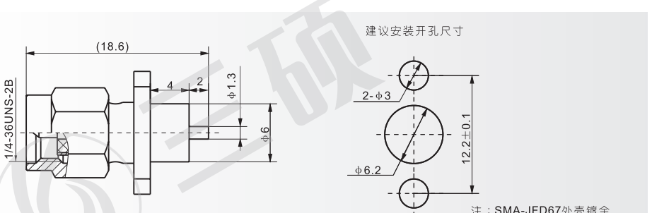
SMA-JFD67 SMA-JFD68G
