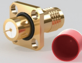
SMA(M)-KFD29(气密封)
